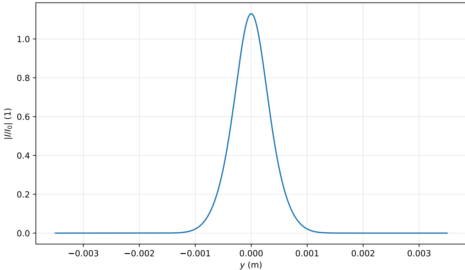
Intensity profile I(x=0, y, z=0.637)/I_0 , \text{Pin}=0.7\text{Pcr} , artificial time
